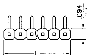
(NO. OF CONTACTS)X1.27
