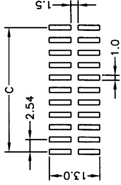
P.C. Board Layout
