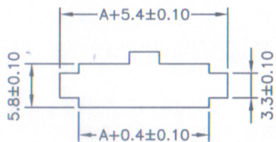
panel hole dimensios
