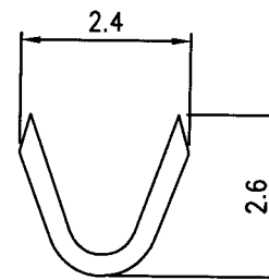
B-B SECTION
