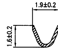
B-B SECTION
