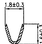
B-B SECTION
