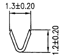
B-B SECTION
